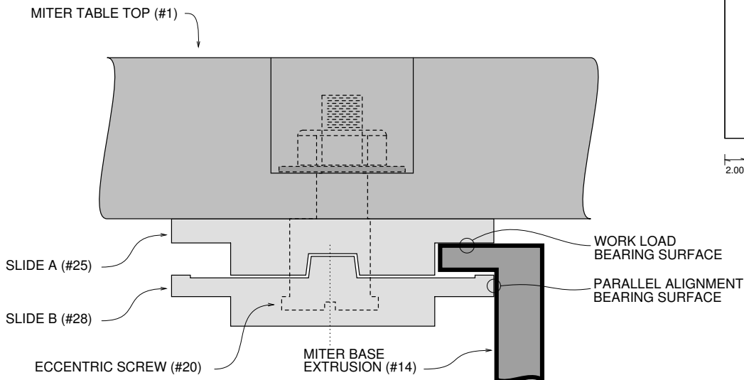
SMT BEARING (NOT TO SCALE)
